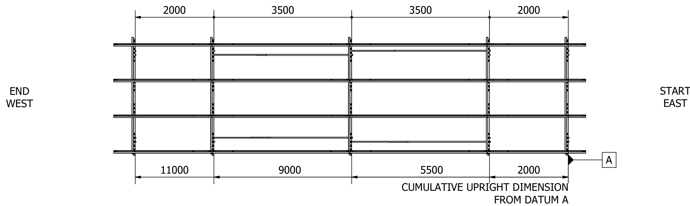
PLAN VIEW SHOWING PILE POSITIONS
