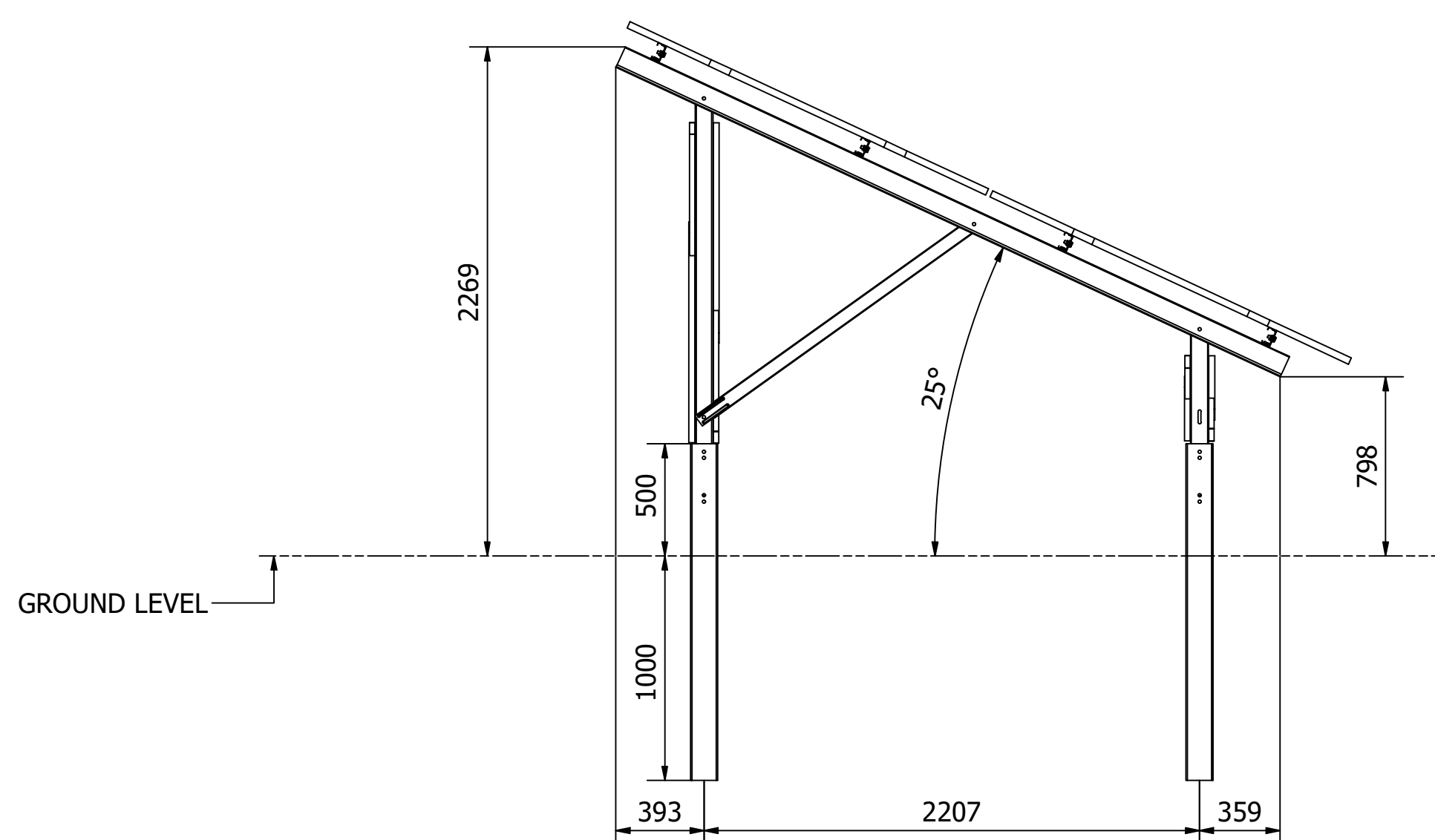
SIDE VIEW NOT TO SCALE SHOW UPRIGHT POSITIONS
