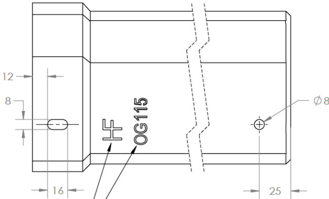
VIEW FROM UNDERSIDE
