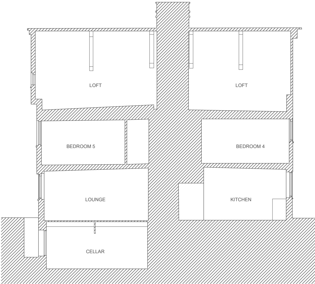
Section BB
