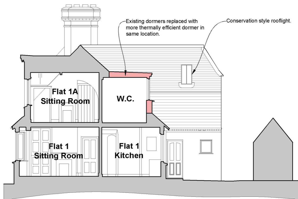
3 Section C-C Proposed 1:100
