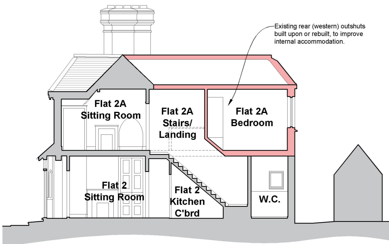
2 Section B-B Proposed 1:100
