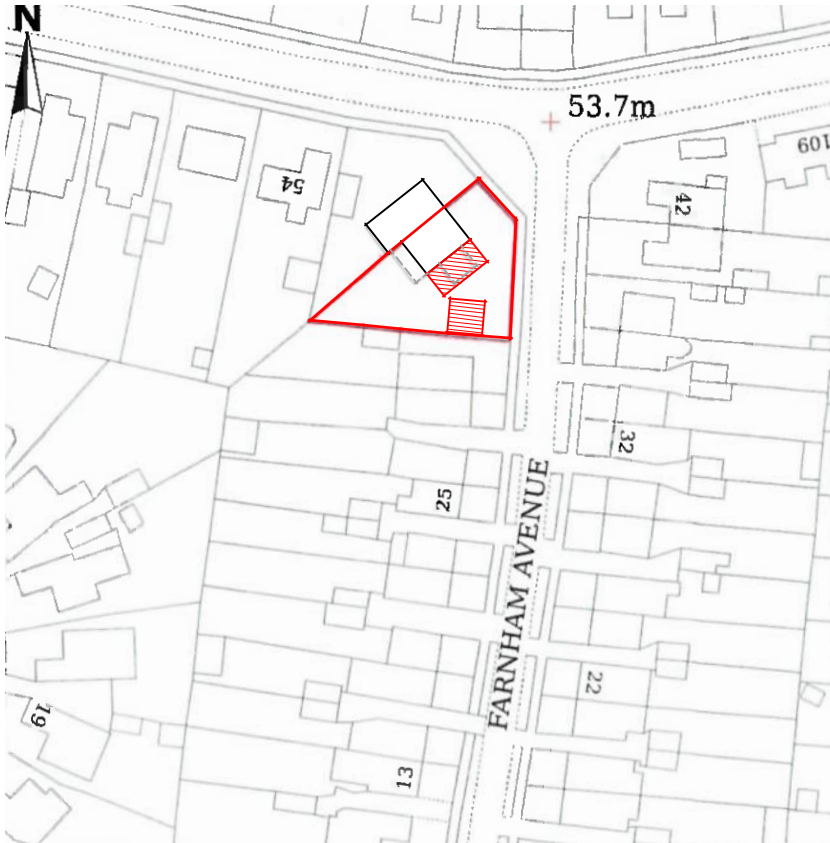
1 Site Location Plan Scale: 1:1250 0 25 50 75 100 m
