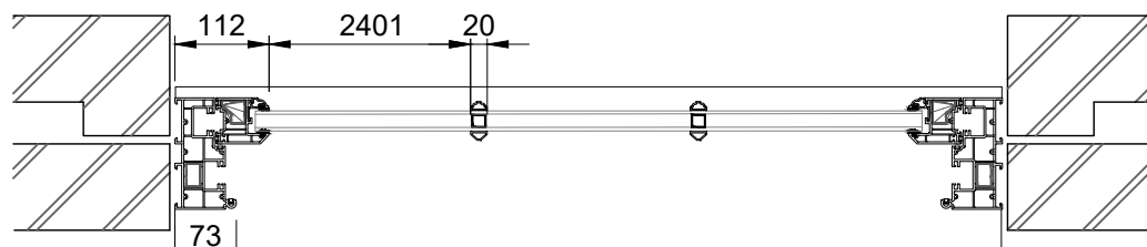
Lower Sash
