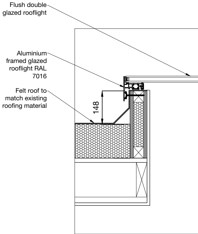
Detailed Section through rooflight. 1:10
