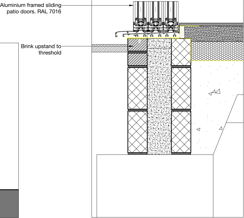
Detailed Section - 1:10
