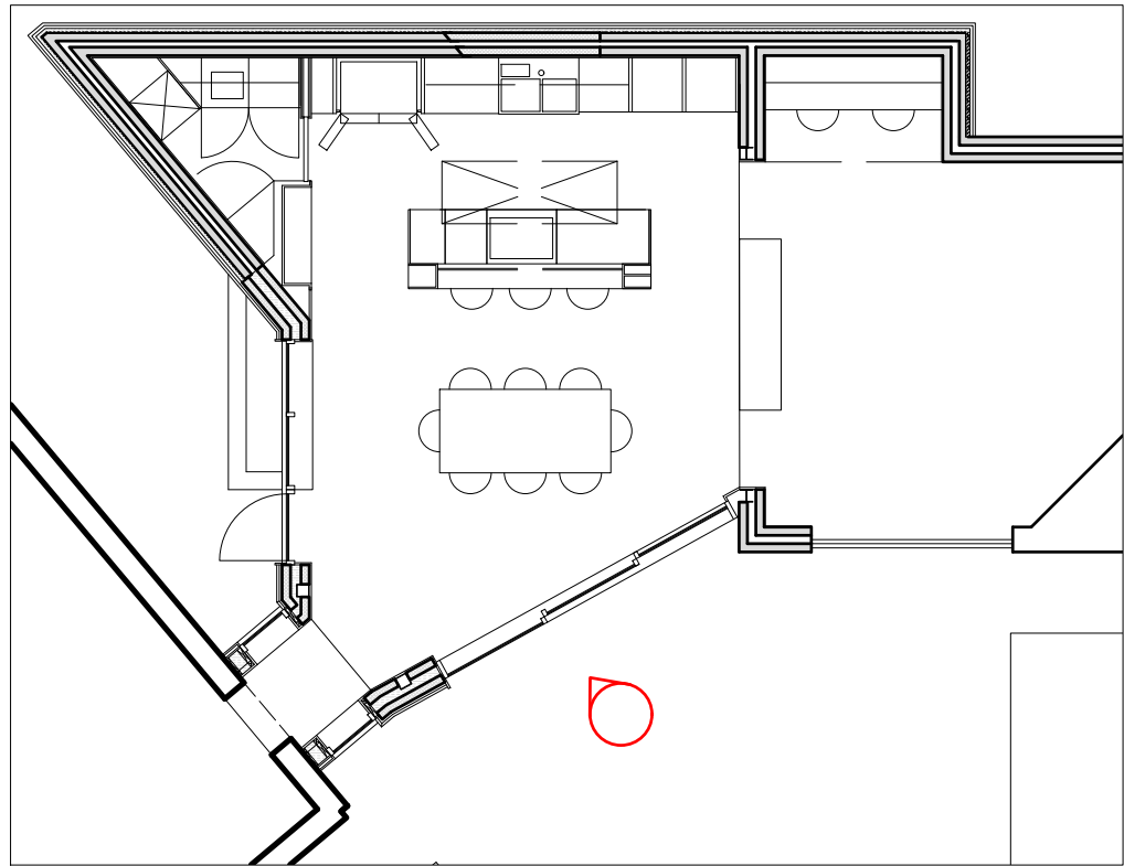
Key Plan - 1:100
