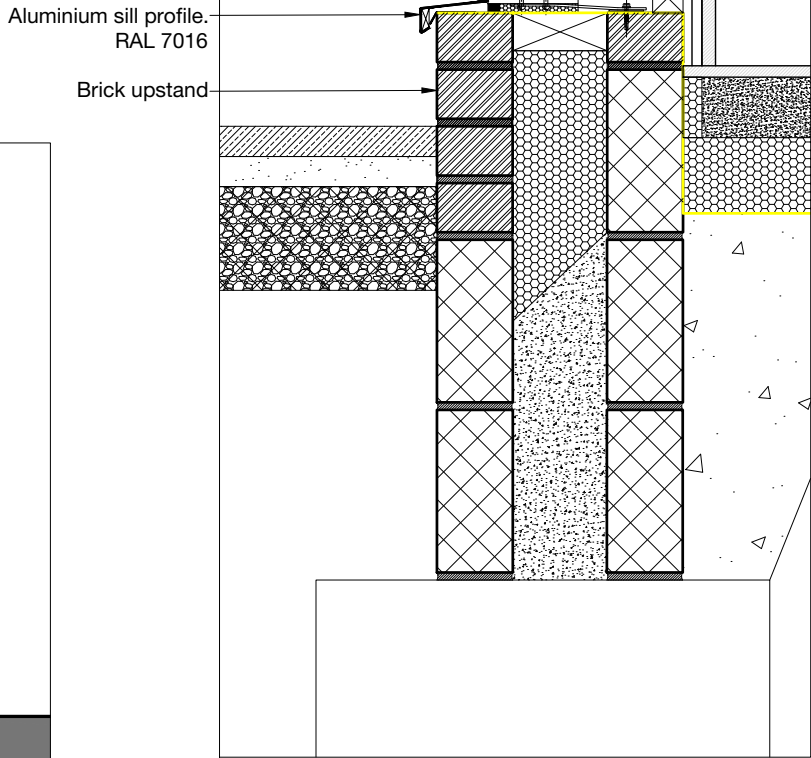
Detailed Section - 1:10
