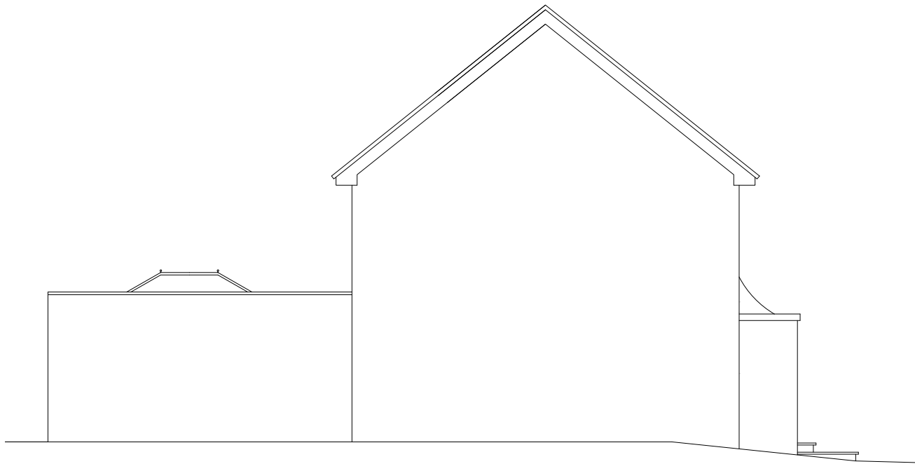
Side Elevation 1:100
