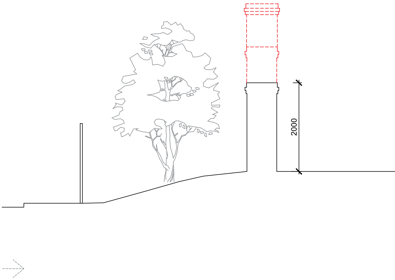
Eastern Section 2 - Proposed (Existing in RED Hatch outline overlay)- 1:50@A0
