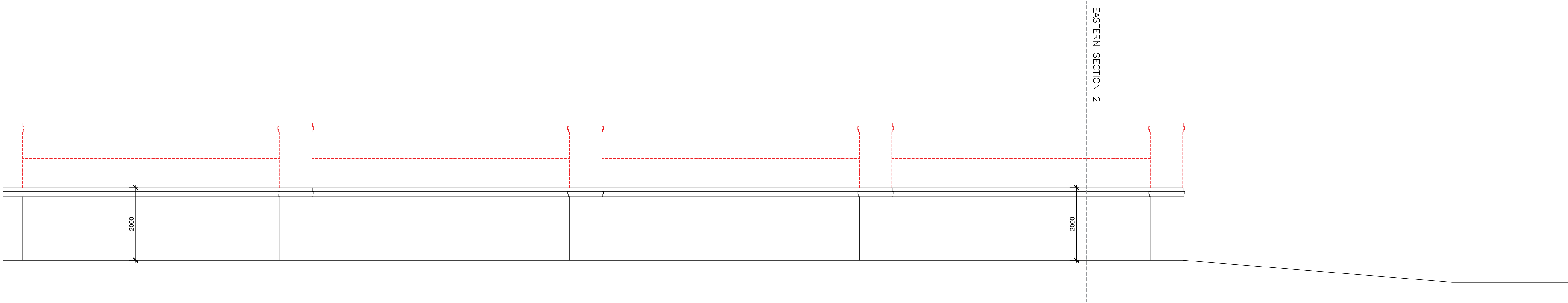
South West Wall Part 2 - Proposed (Existing in RED Hatch outline overlay)- 1:50@A0
