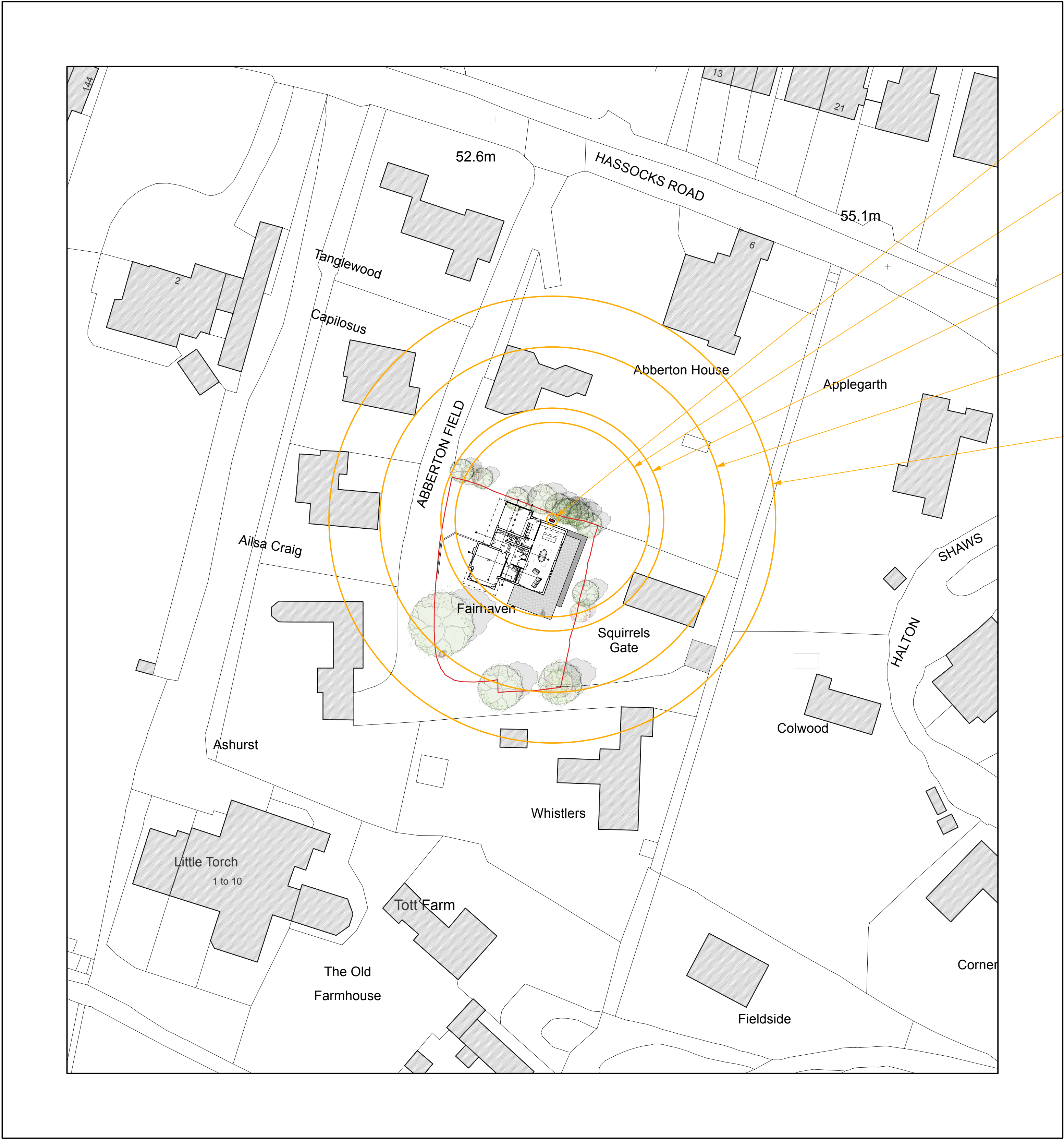
Block Plan 1:500
