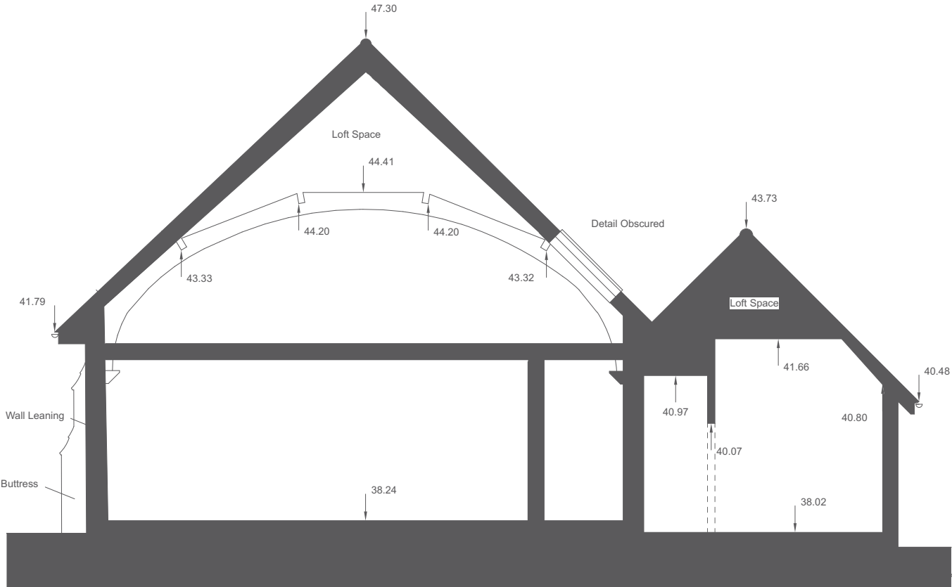
01 - PROPOSED SECTION 1
