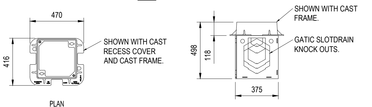
350 ACCESS BOX SECTION AND PLAN DETAILS NTS
