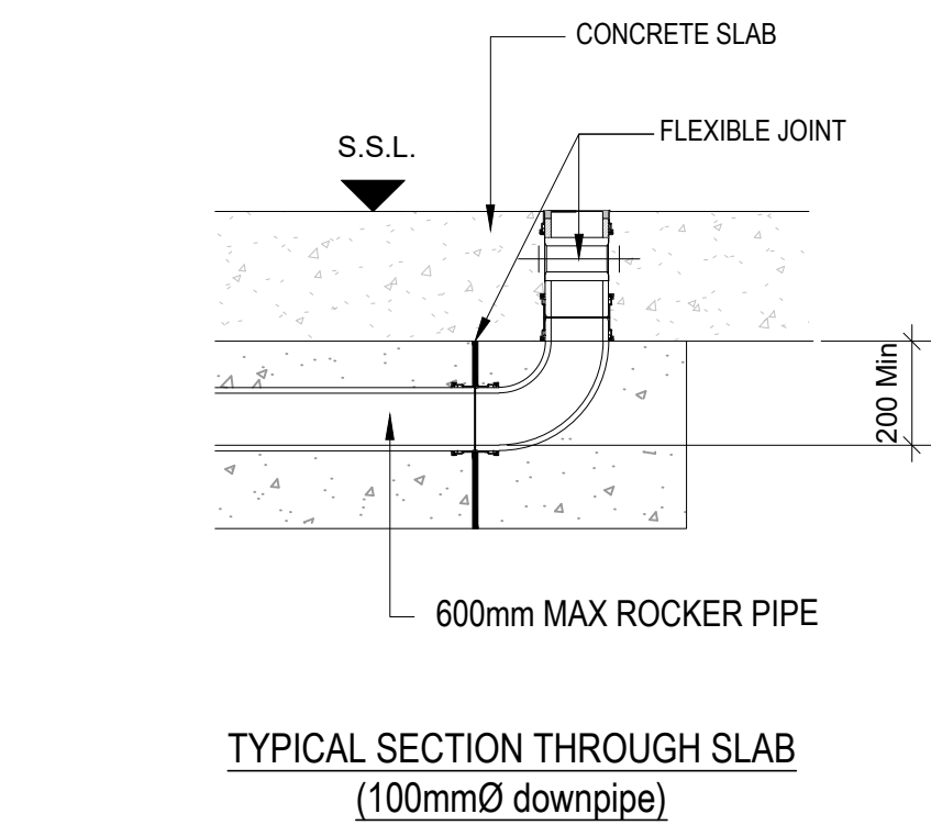
TYPICAL SVP CONNECTION TO MAIN RUN
