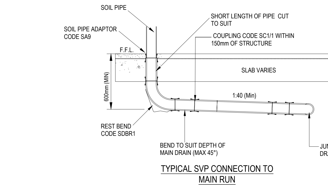
DRAINAGE UNDER BUILDINGS
