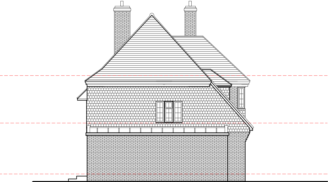
B) Existing Side Elevation
