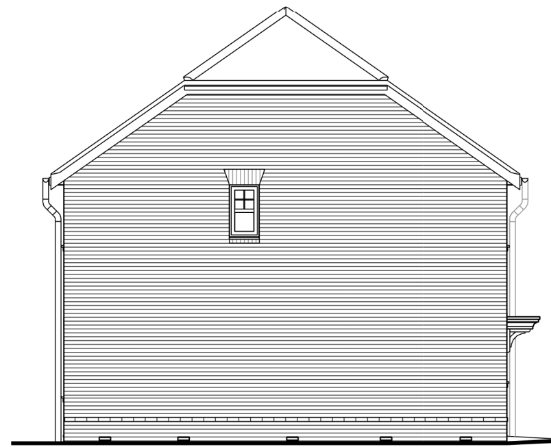
Left Elevation
