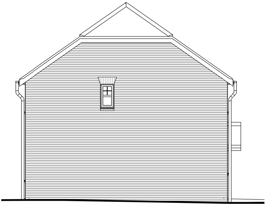
Left Elevation
