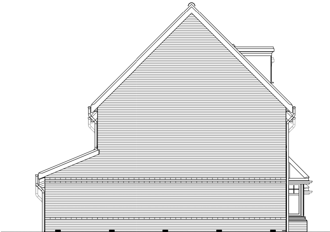
Left Elevation
