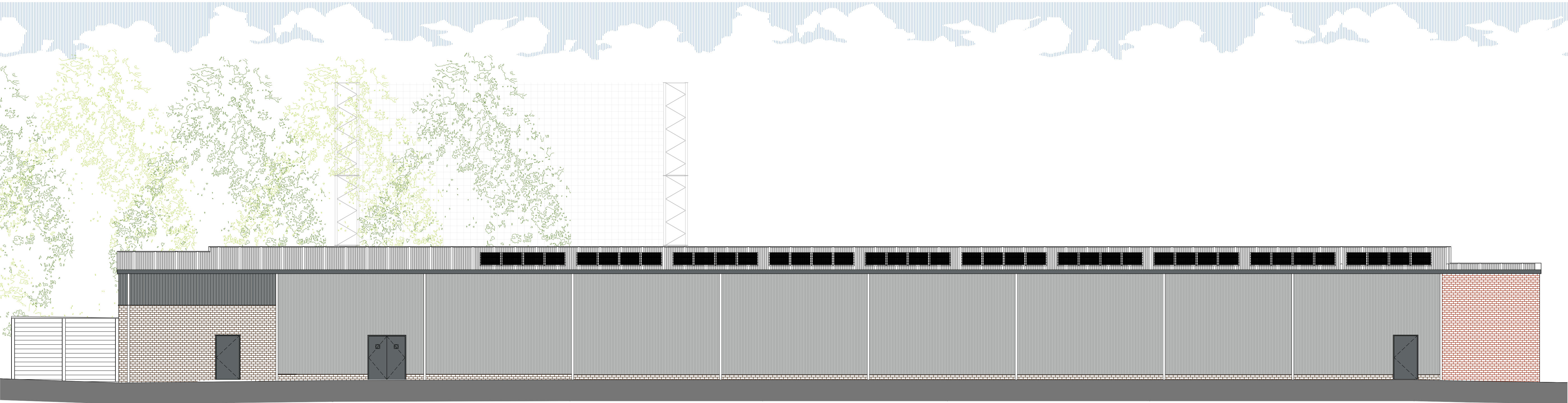
PROPOSED ELEVATION C | NORTH scale 1:100
