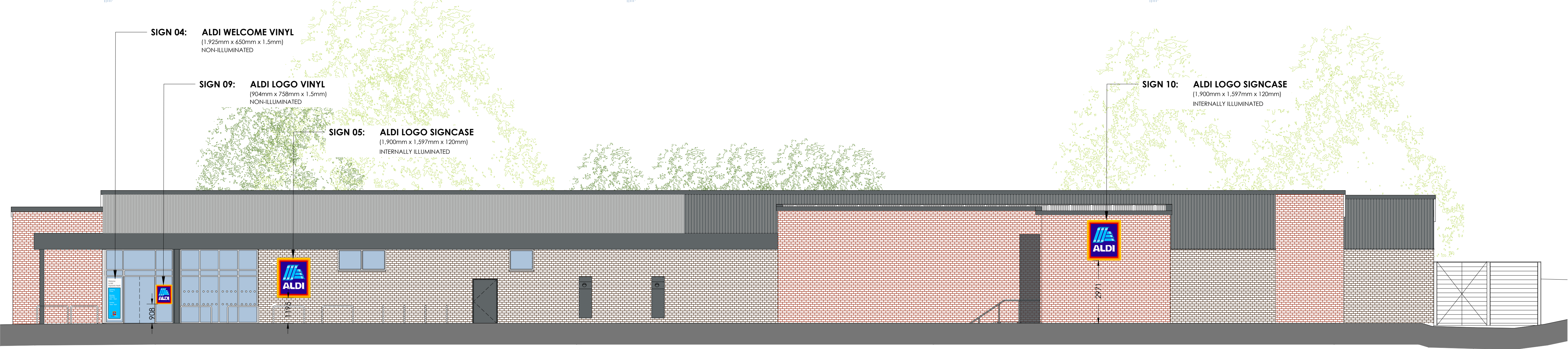
PROPOSED ELEVATION A | SOUTH scale 1:100
