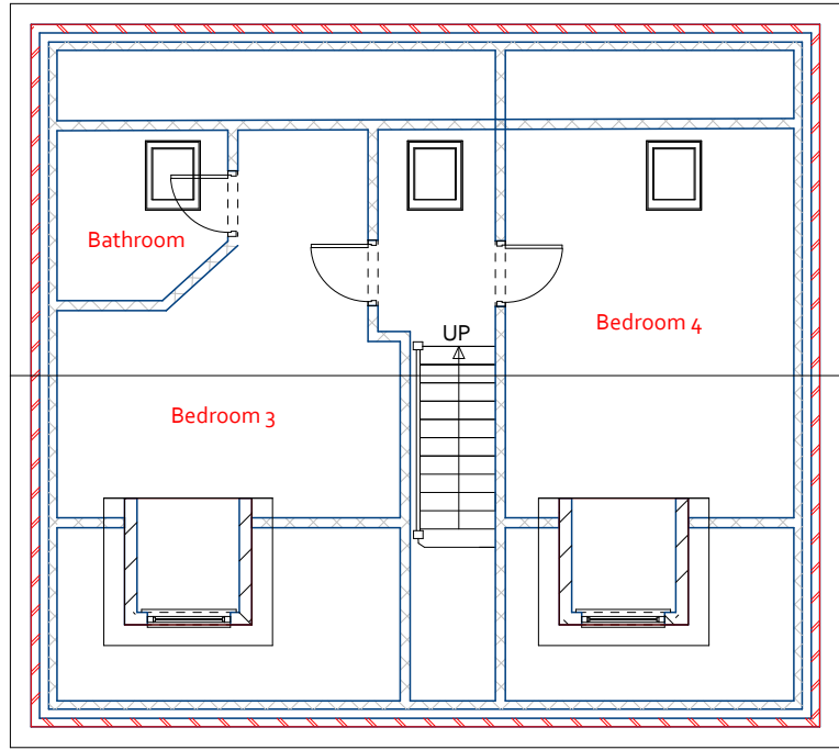
Second floor
