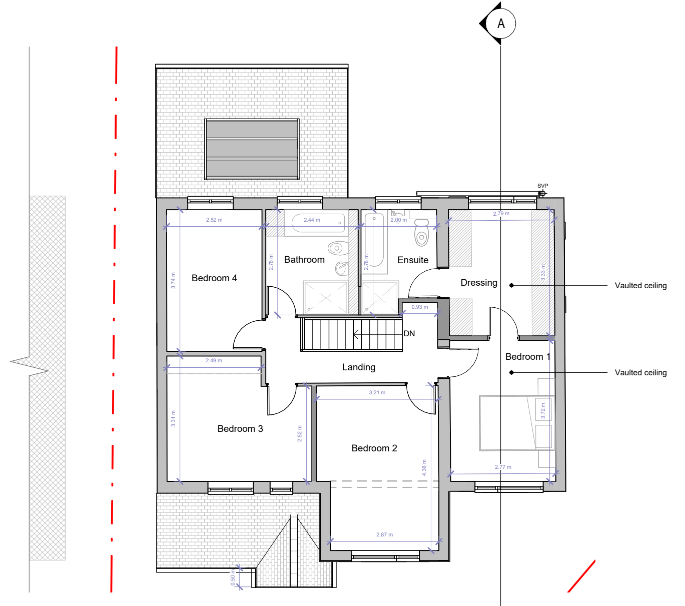
First Floor
