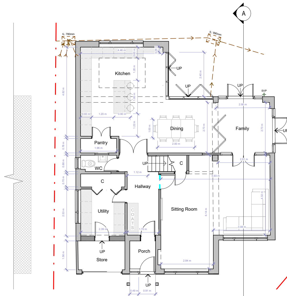
Ground Floor
