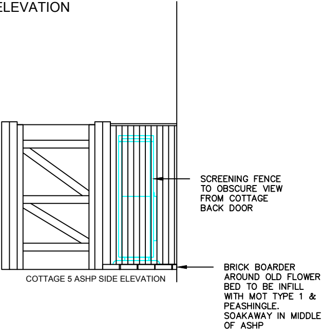
COTTAGE 5 ASHP SIDE ELEVATION
