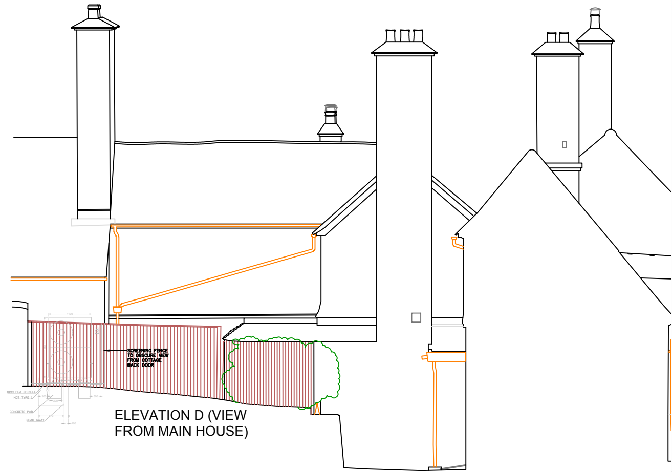
COTTAGE 5 ASHP ELEVATION
