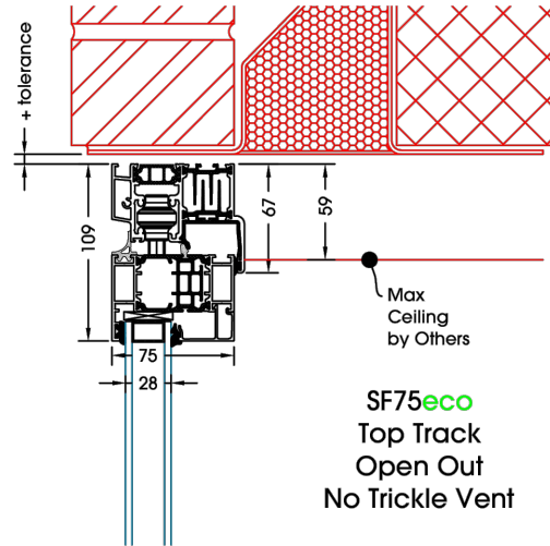
TYPICAL TOP SECTION ELEVATION
