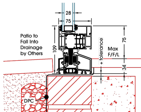
TYPICAL BOTTOM SECTION ELEVATION
