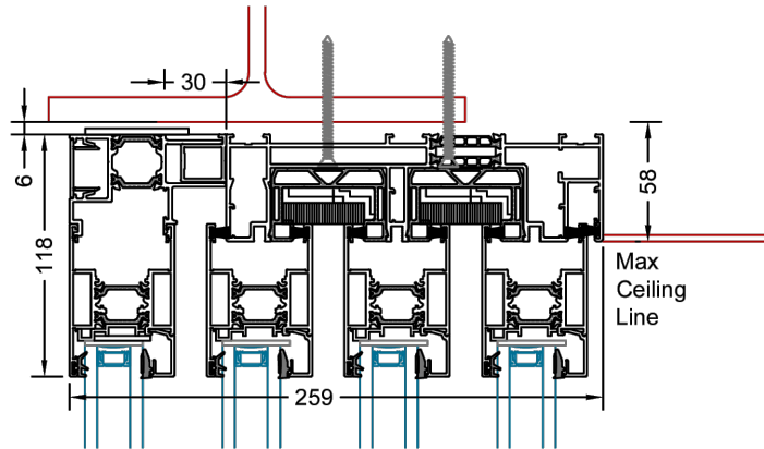
TYPICAL TOP SECTION ELEVATION
