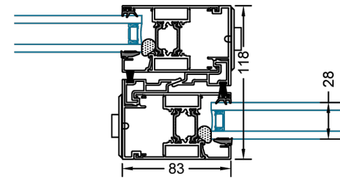
TYPICAL MULLION SECTION FROM ABOVE
