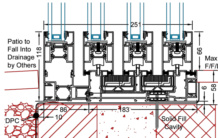
TYPICAL BOTTOM SECTION ELEVATION
