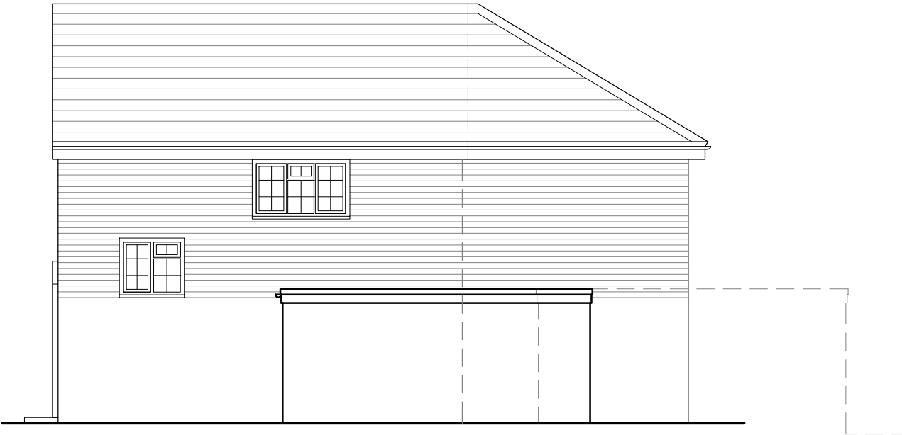
WEST ELEVATION
