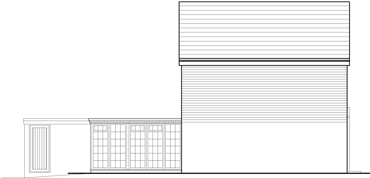
EAST ELEVATION
