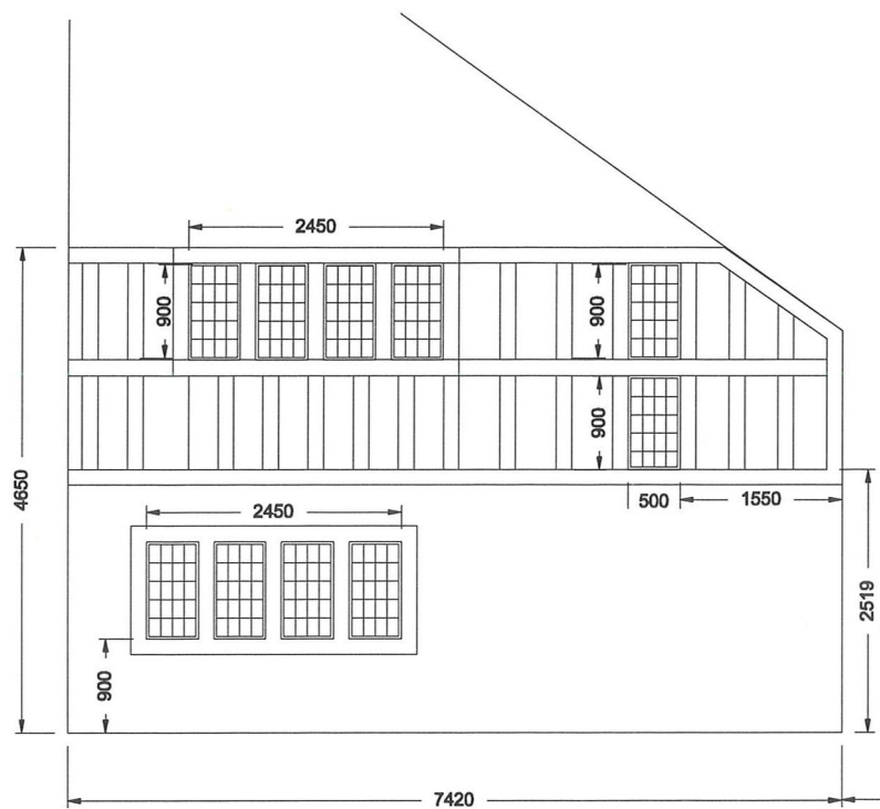
Front Elevation Scale 1 : 50 when printed A4
