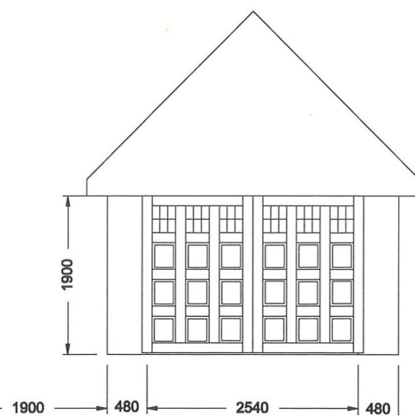
Position of car port relative to main house showing side opening wooden doors
