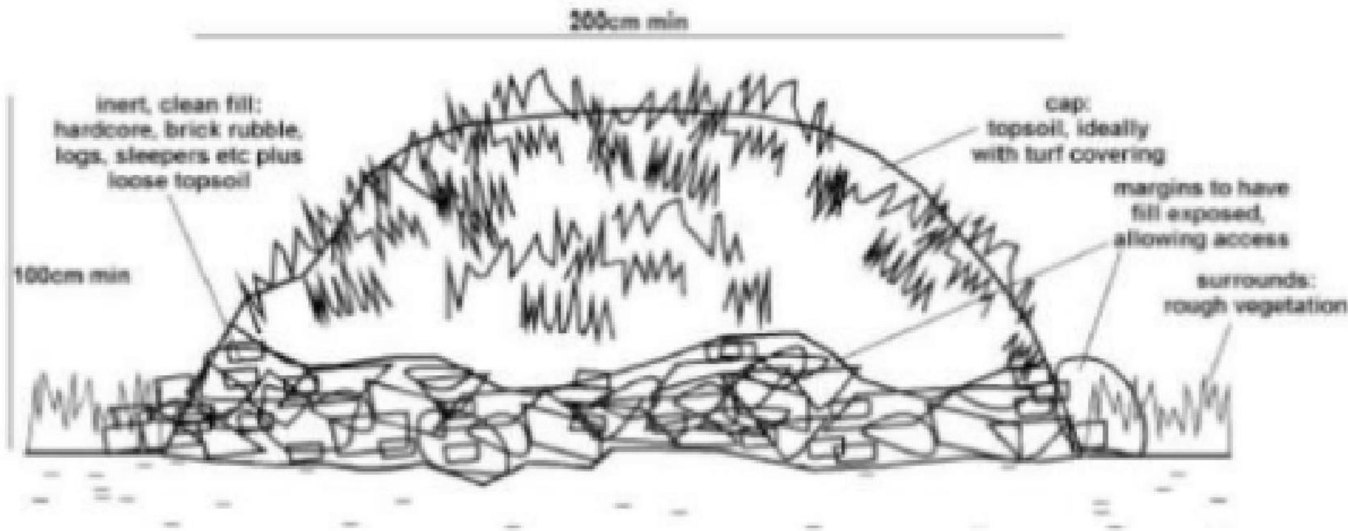
Figure 17. Reptile hibernaculum design as provided in HART (2009).
