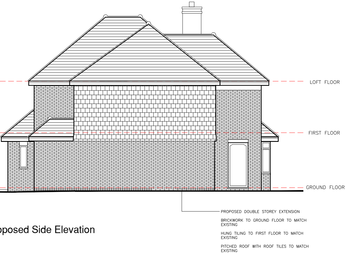
D) Proposed Side Elevation
