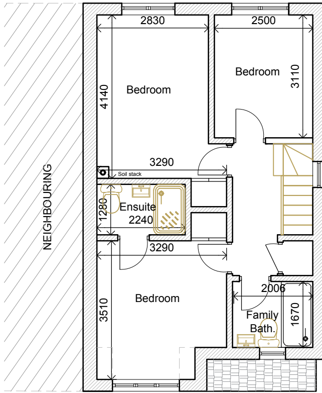
02 First floor plan - As Existing 2000 1:100 (at A3)
