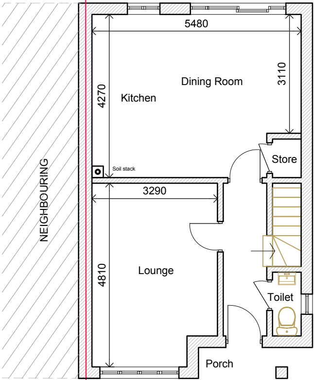
01 Ground Floor Plan - As Existing 2000 1:100 (at A3)
