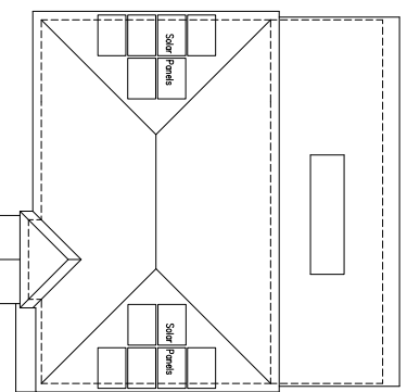
Proposed roof plan @ 1:100
