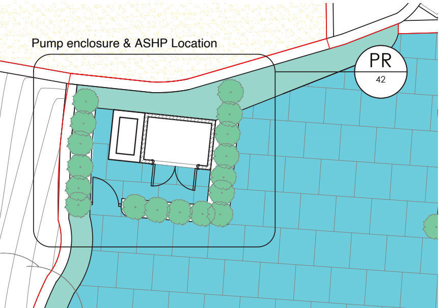
Extracted 27900_PR_40 - Plan of pump enclosure & hedging
