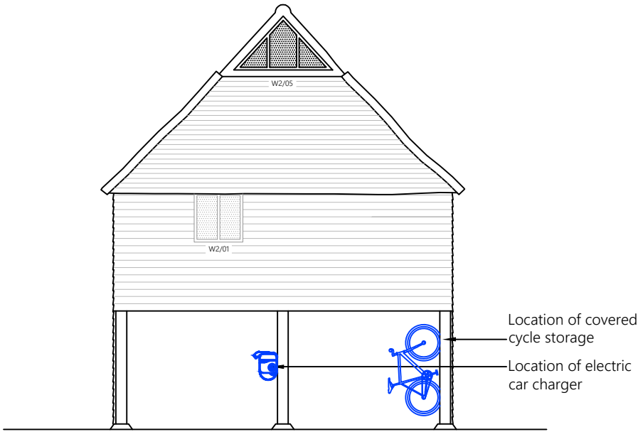
South Elevation 1:50
