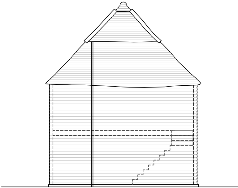
North Elevation 1:50
