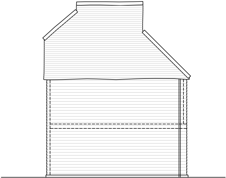
West Elevation 1:50
