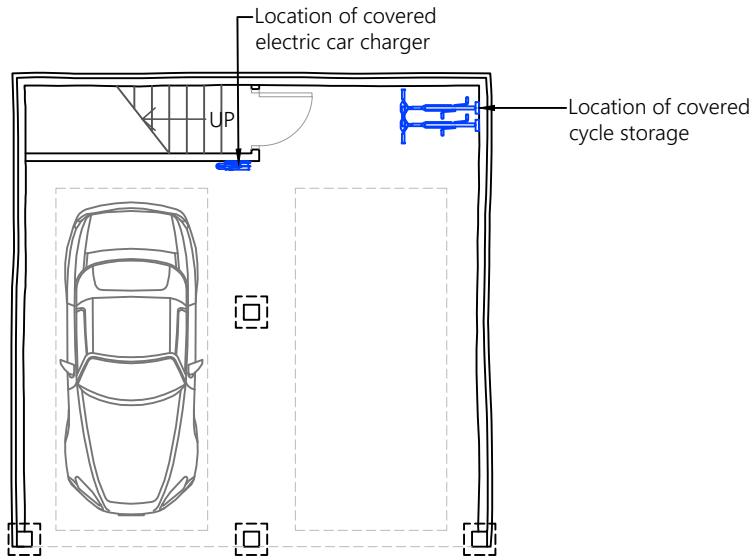
Ground Floor Plan 1:50
