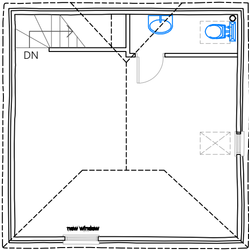
First Floor Plan 1:50
