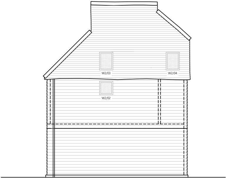
East Elevation 1:50
