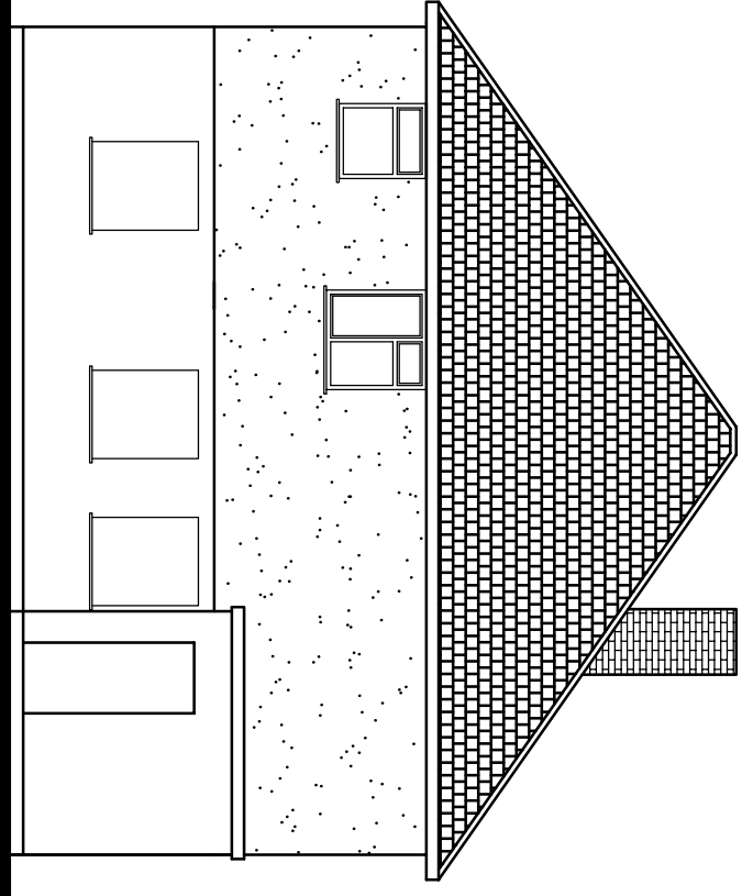
Proposed Rear (East) Elevation
