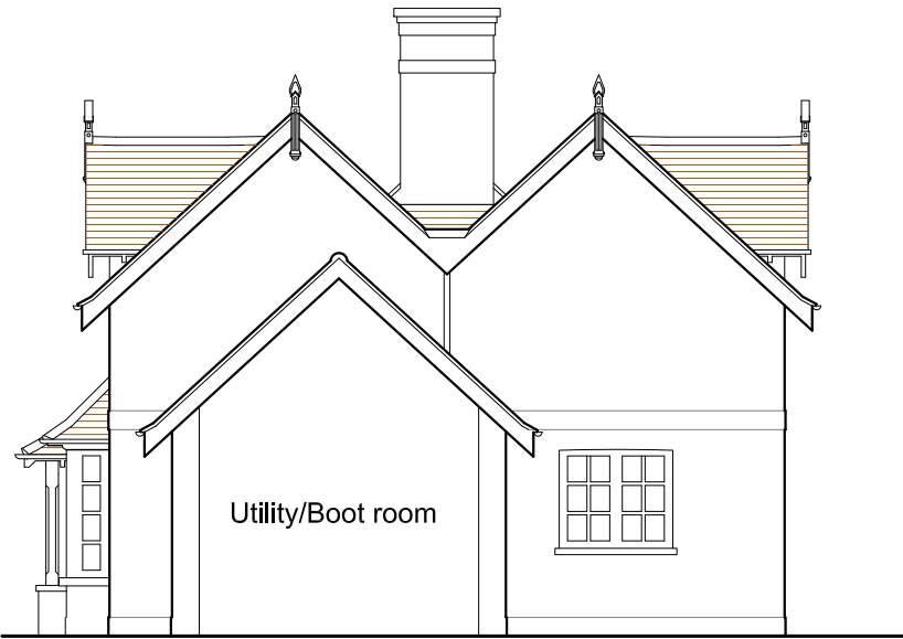
Proposed Section / Side Elevation - NE
