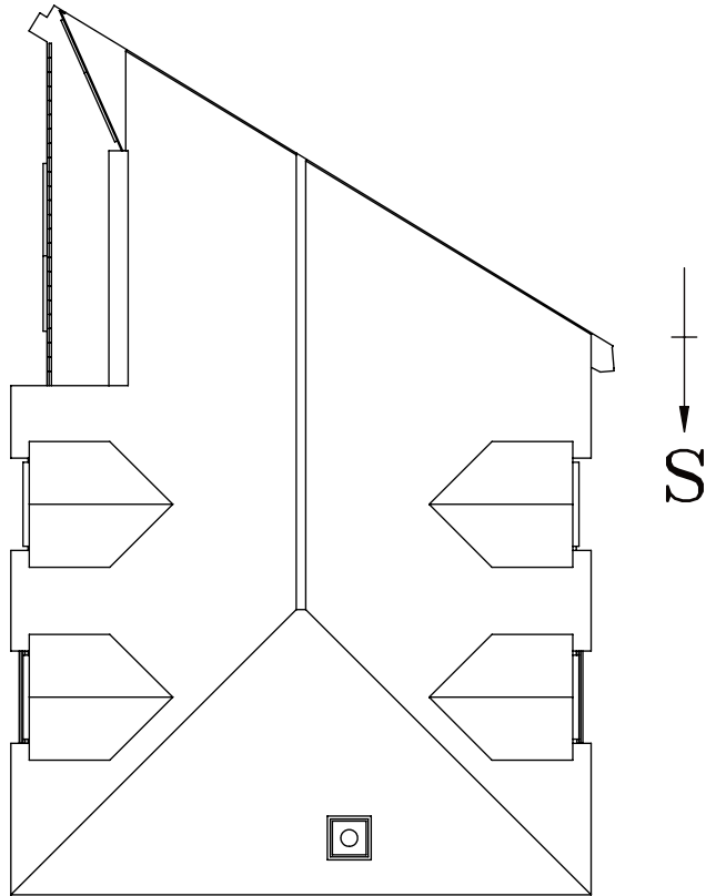
Partial View Of Plan View
