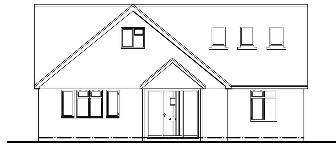
NW ELEVATION
