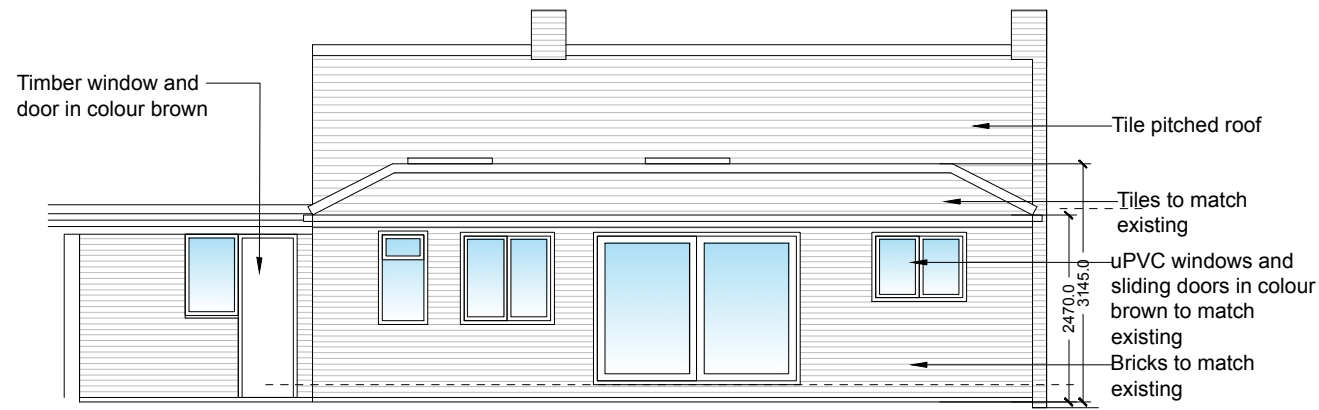
Rear (South) Elevation as proposed
