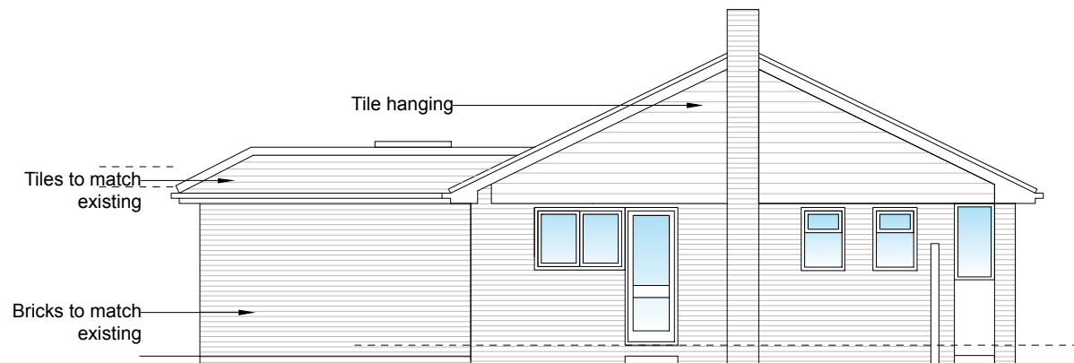
Side (East) Elevation as proposed
