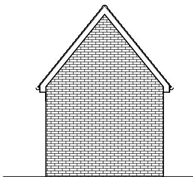
Garage Rear Elevation Scale 1:100
