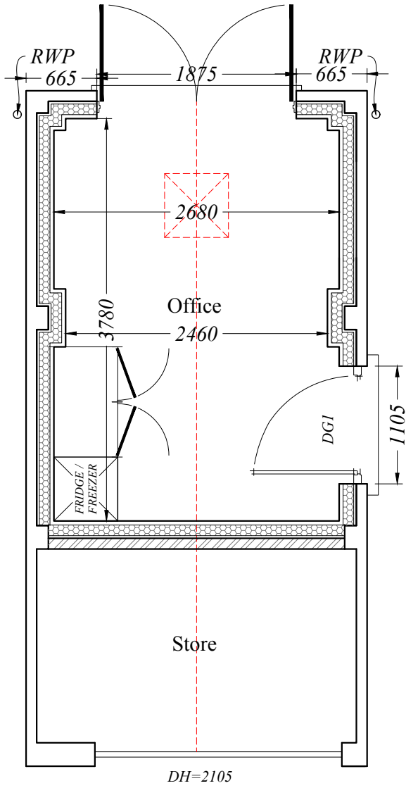
Garage Floor Plan Scale 1:50
