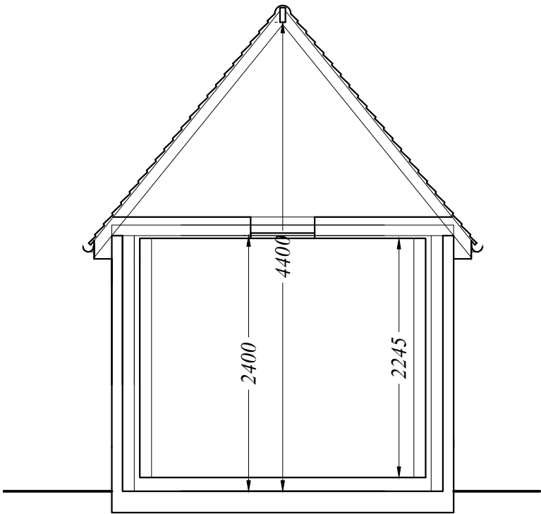
Section B-B Scale 1:50
