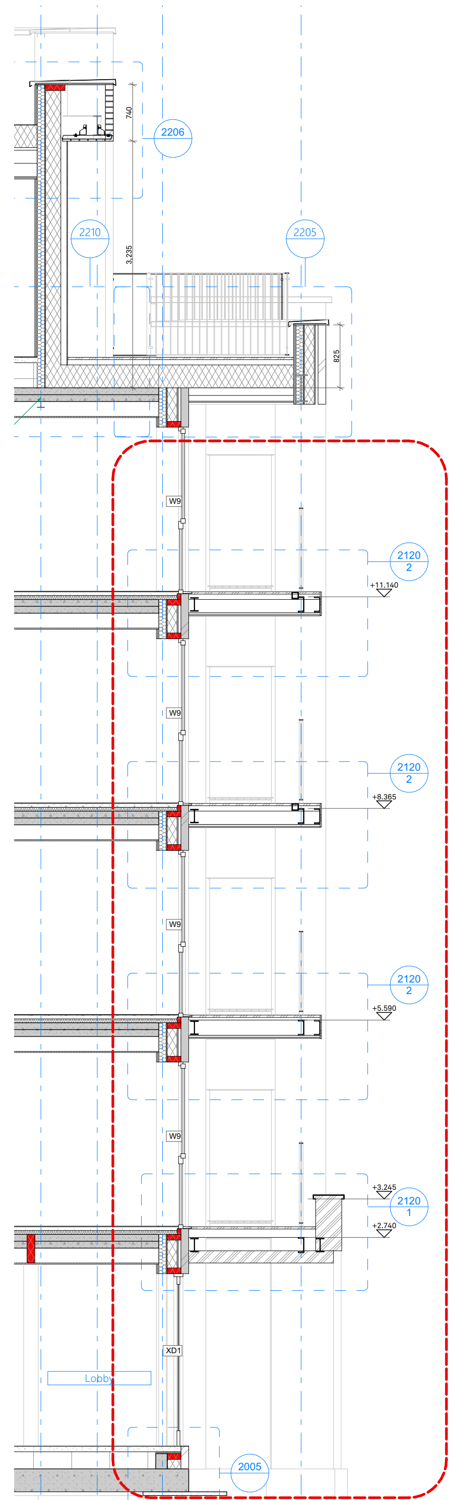
S-02 Building Section
