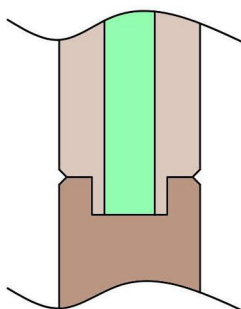
bevelled (Tongue & groove) moulding with flush panels
