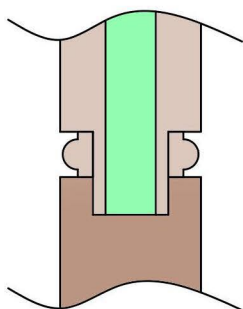
Pencil bead moulding with flush panels
