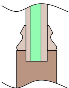
Trimmed ogee moulding with flat panels
