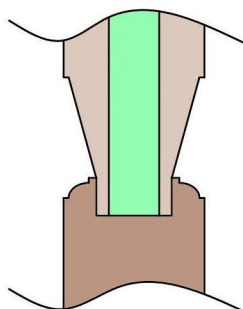
Ovolo moulding with raised & fielded panels both sides
