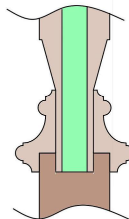
Bolection moulding with raised & fielded panels
