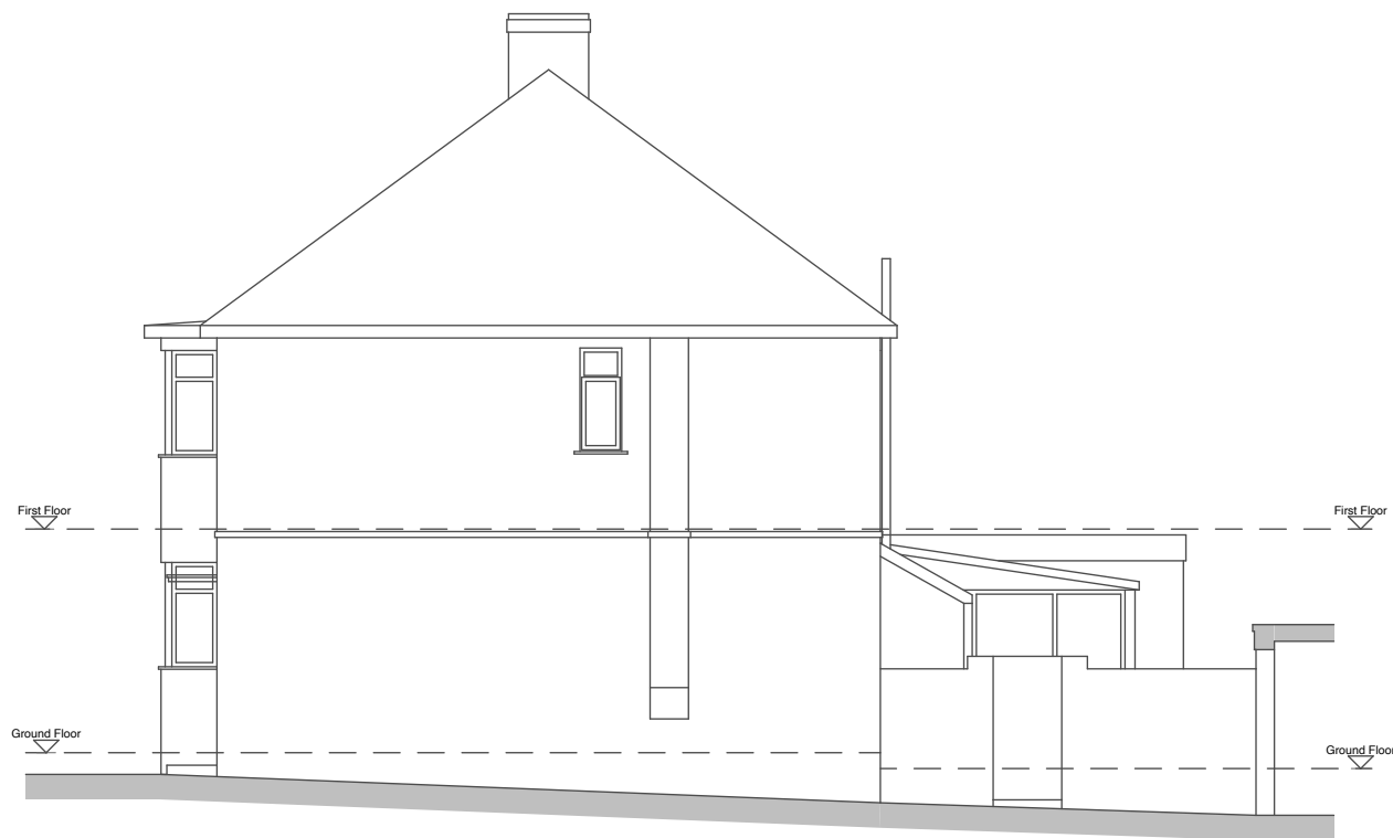
NORTH ELEVATION 1:100
