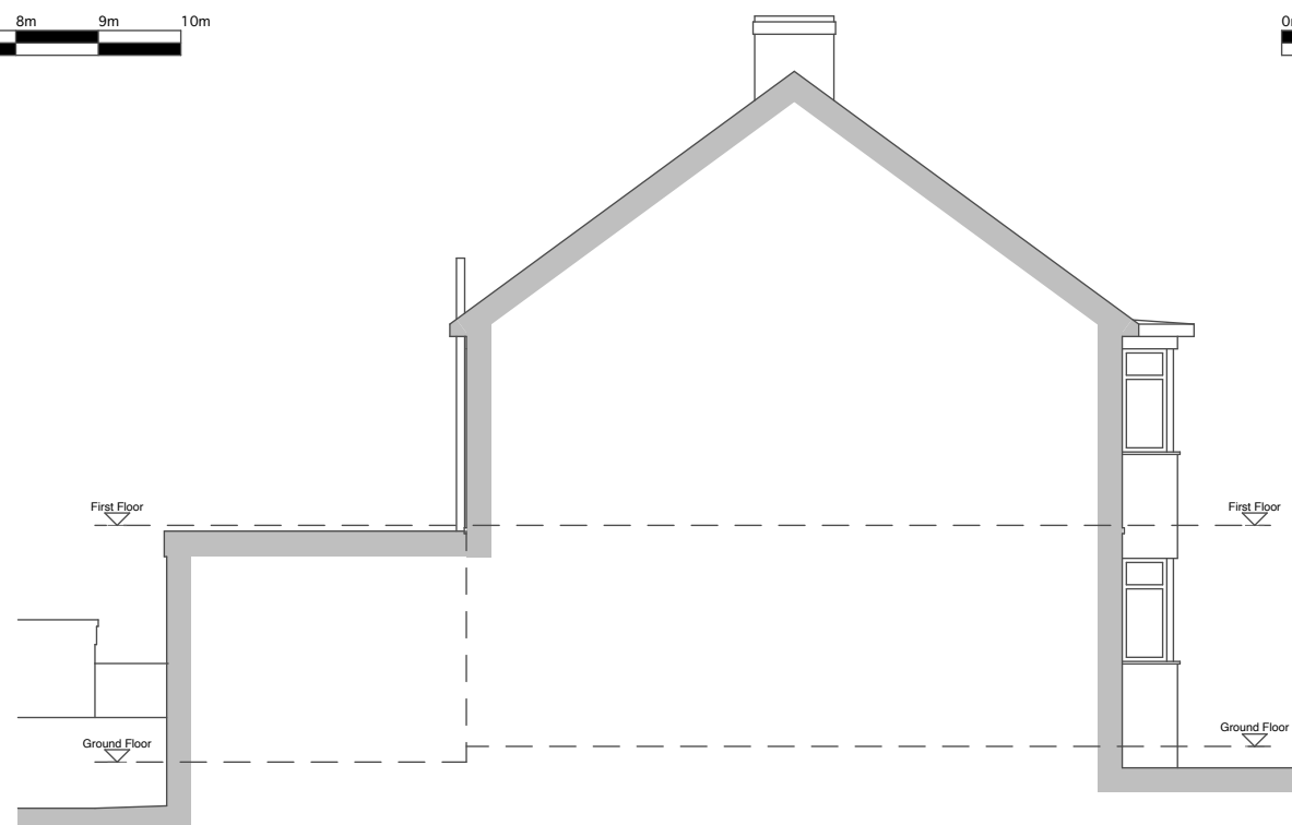
SOUTH SECTION-ELEVATION 1:100
