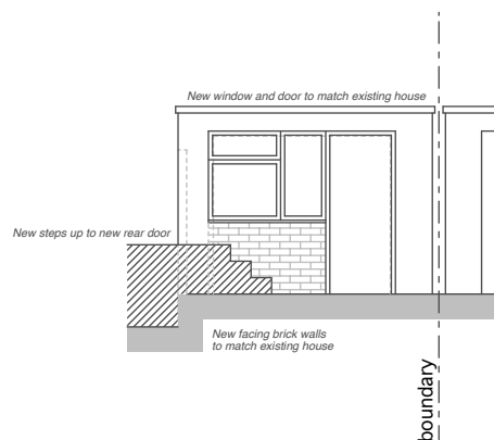
GARAGE ELEVATION
