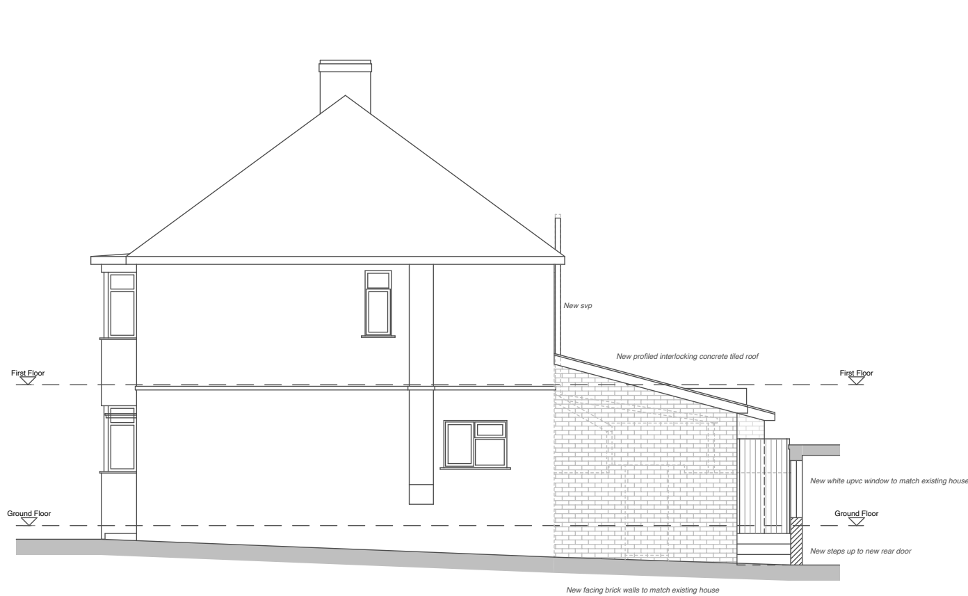
NORTH ELEVATION 1:100
