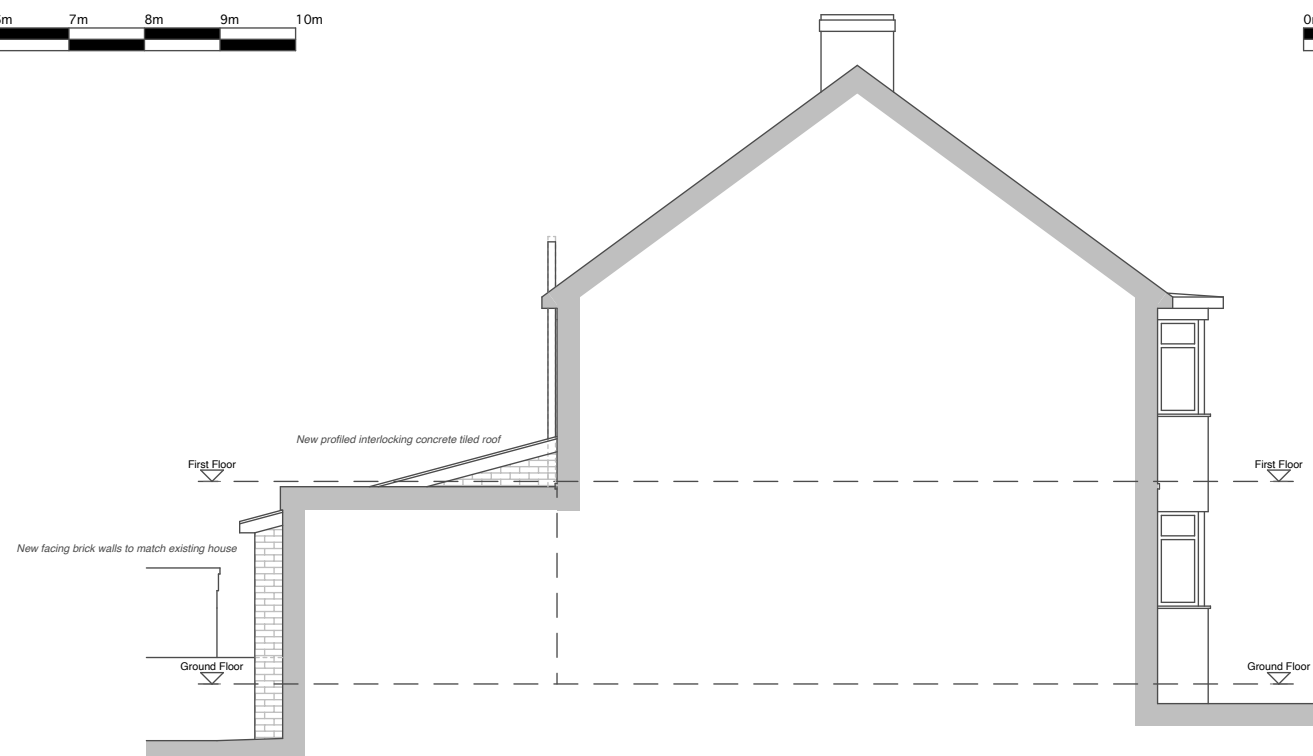
SOUTH SECTION-ELEVATION 1:100
