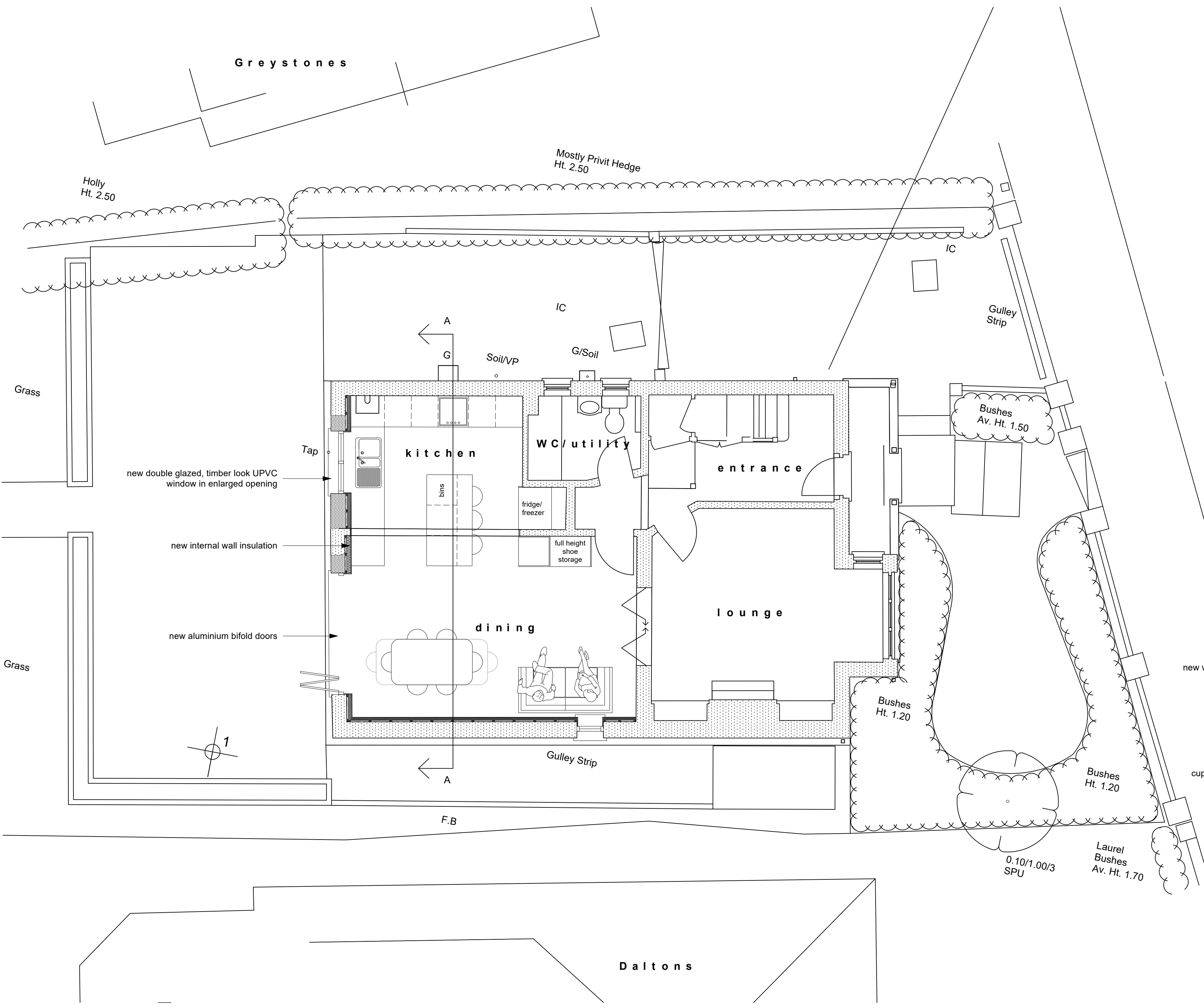
ground floor and site plan
