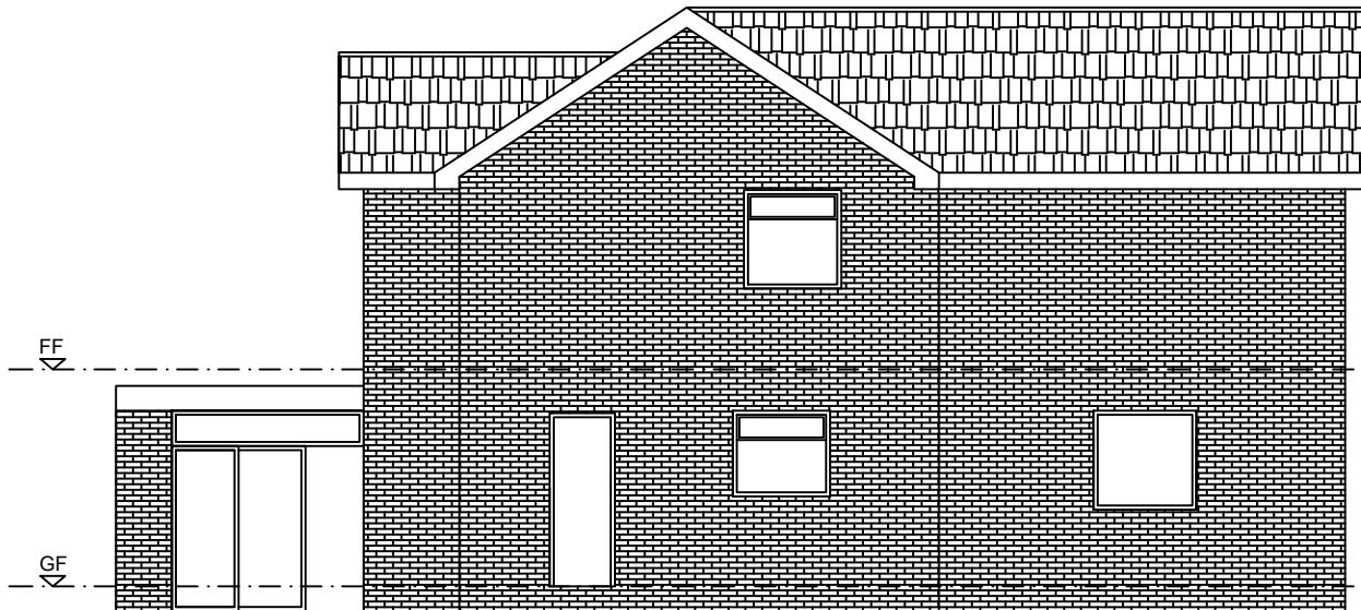
SIDE (EAST) ELEVATION
