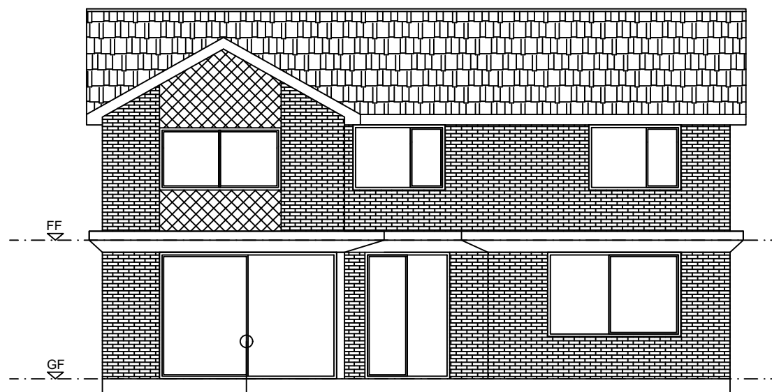
REAR ELEVATION
