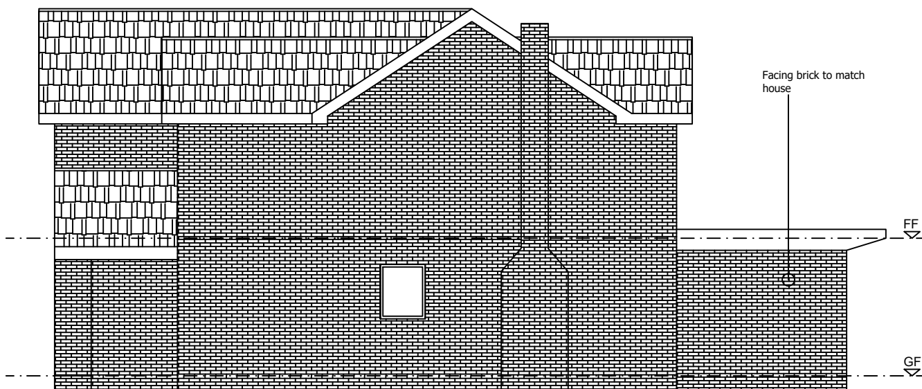
SIDE (WEST) ELEVATION
