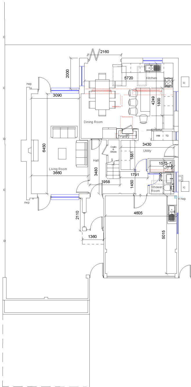
Proposed Ground Floor Plan 1:50
