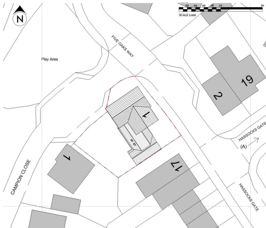
Block plan
