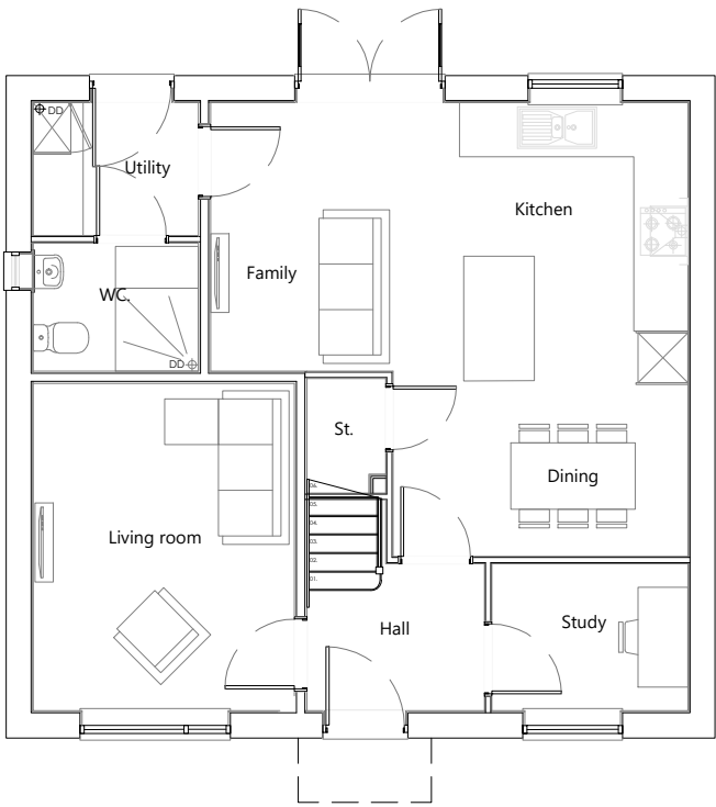
Ground Floor Plan Plot 195 - Brampton SU
